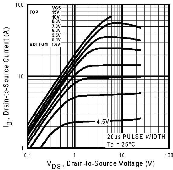
Fig 1. Typical Output Characteristics, TJ=25
